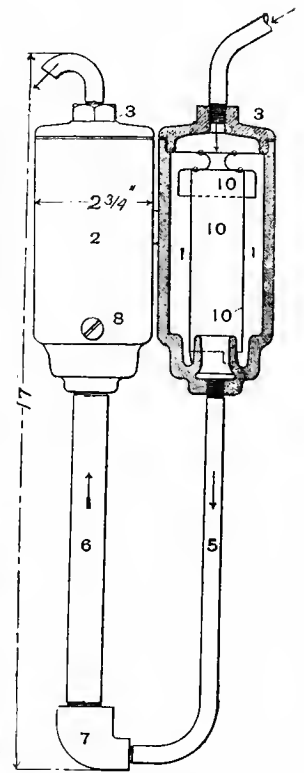
Fig. 3124. Sectional Elevation. MERCURIAL SAFETY-VALVE.
